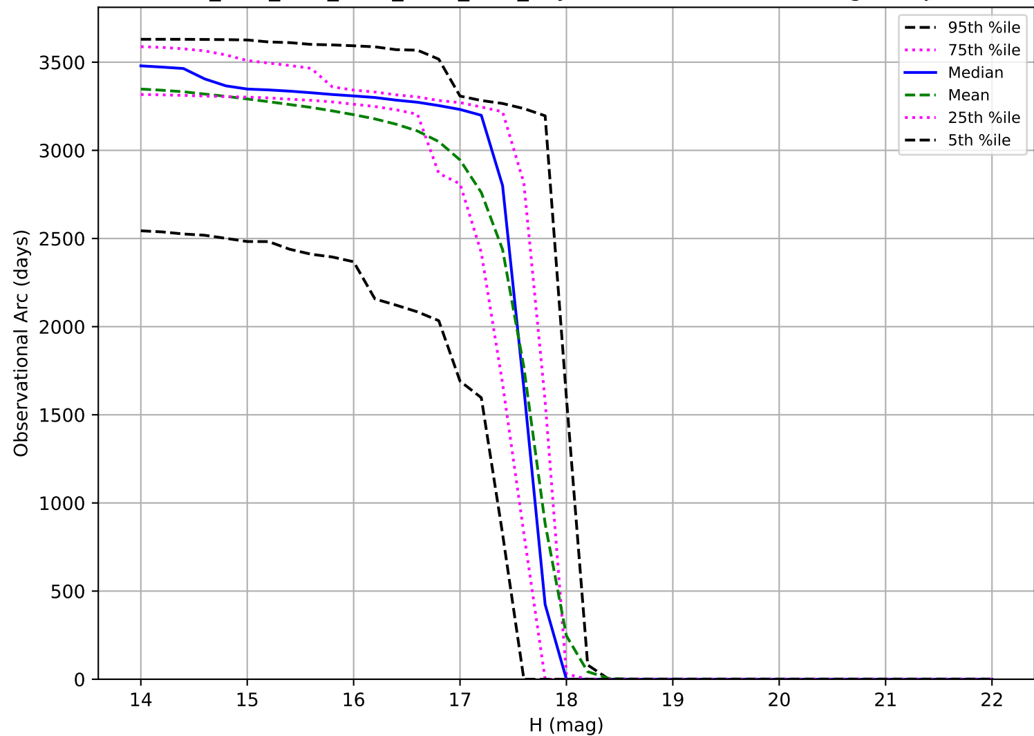
ddf_acor_sf15_lsf40_lsr20_v3.4_10yrs: Observational Arc Length Trojan
