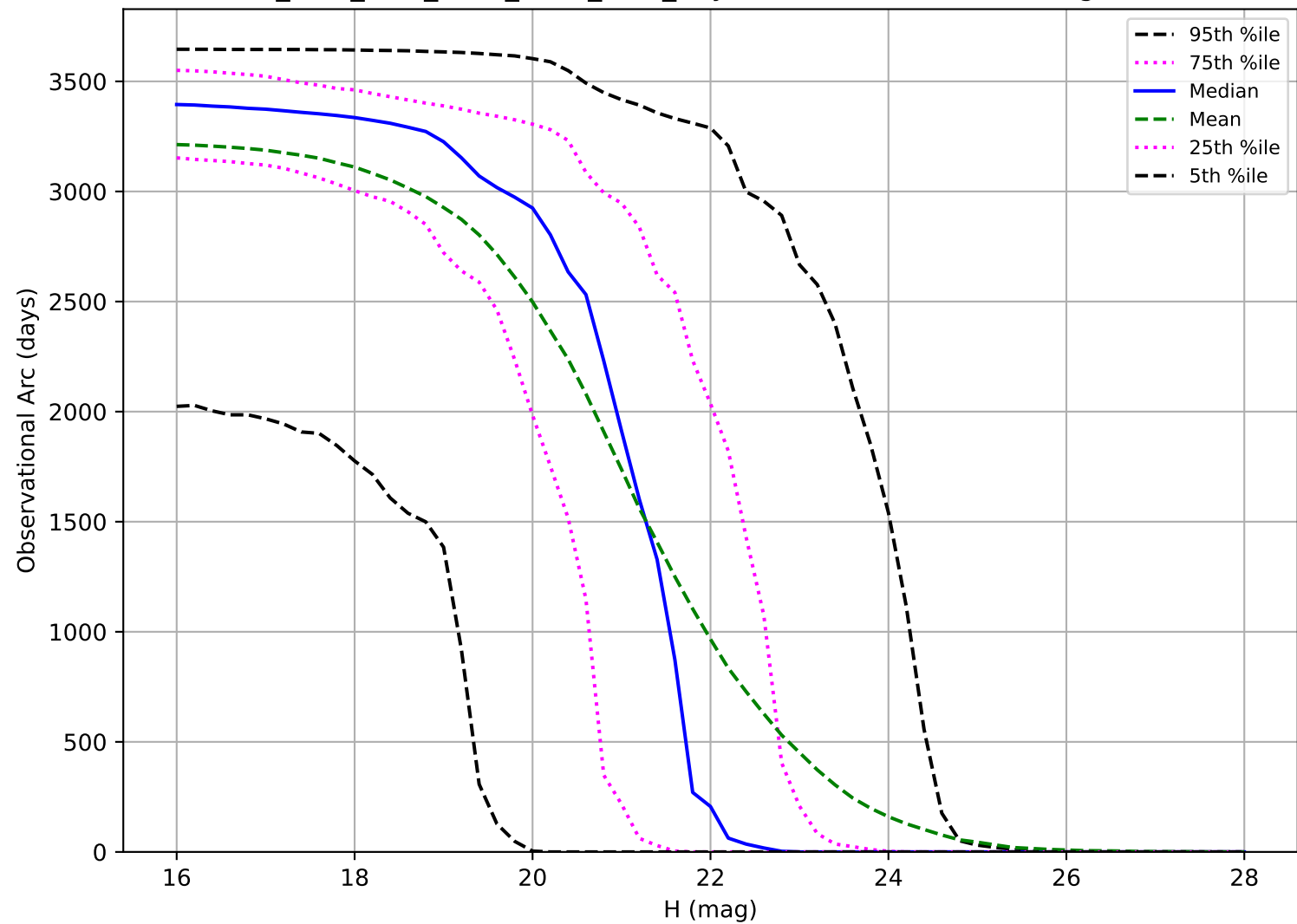
ddf_acor_sf15_lsf40_lsr20_v3.4_10yrs: Observational Arc Length PHA
