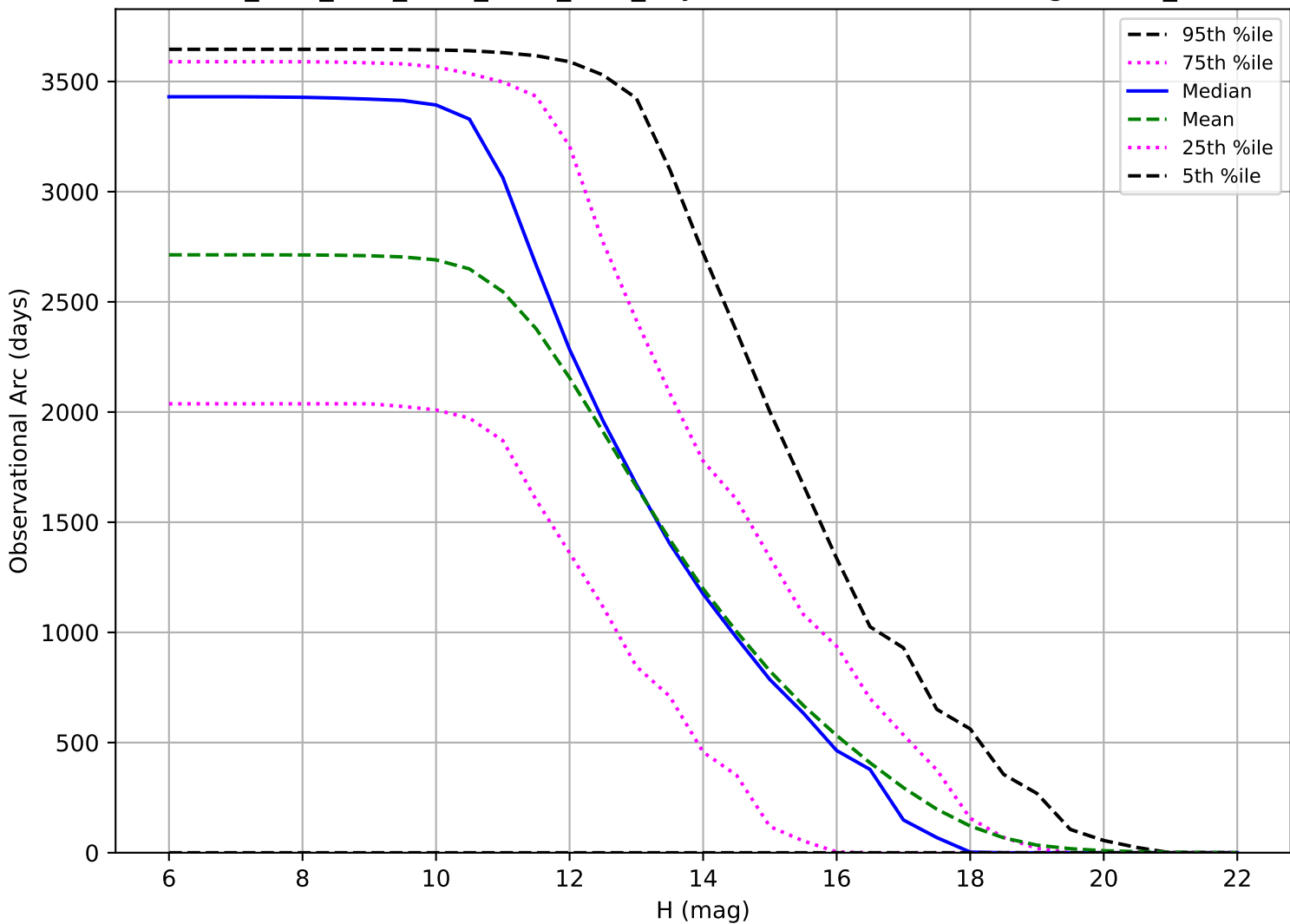
ddf_acor_sf15_lsf40_lsr20_v3.4_10yrs: Observational Arc Length OCC_r5
