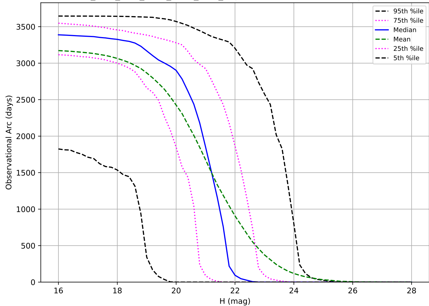
ddf_acor_sf15_lsf40_lsr20_v3.4_10yrs: Observational Arc Length NEO
