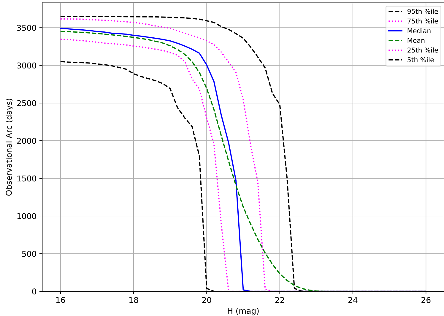
ddf_acor_sf15_lsf40_lsr20_v3.4_10yrs: Observational Arc Length MBA
