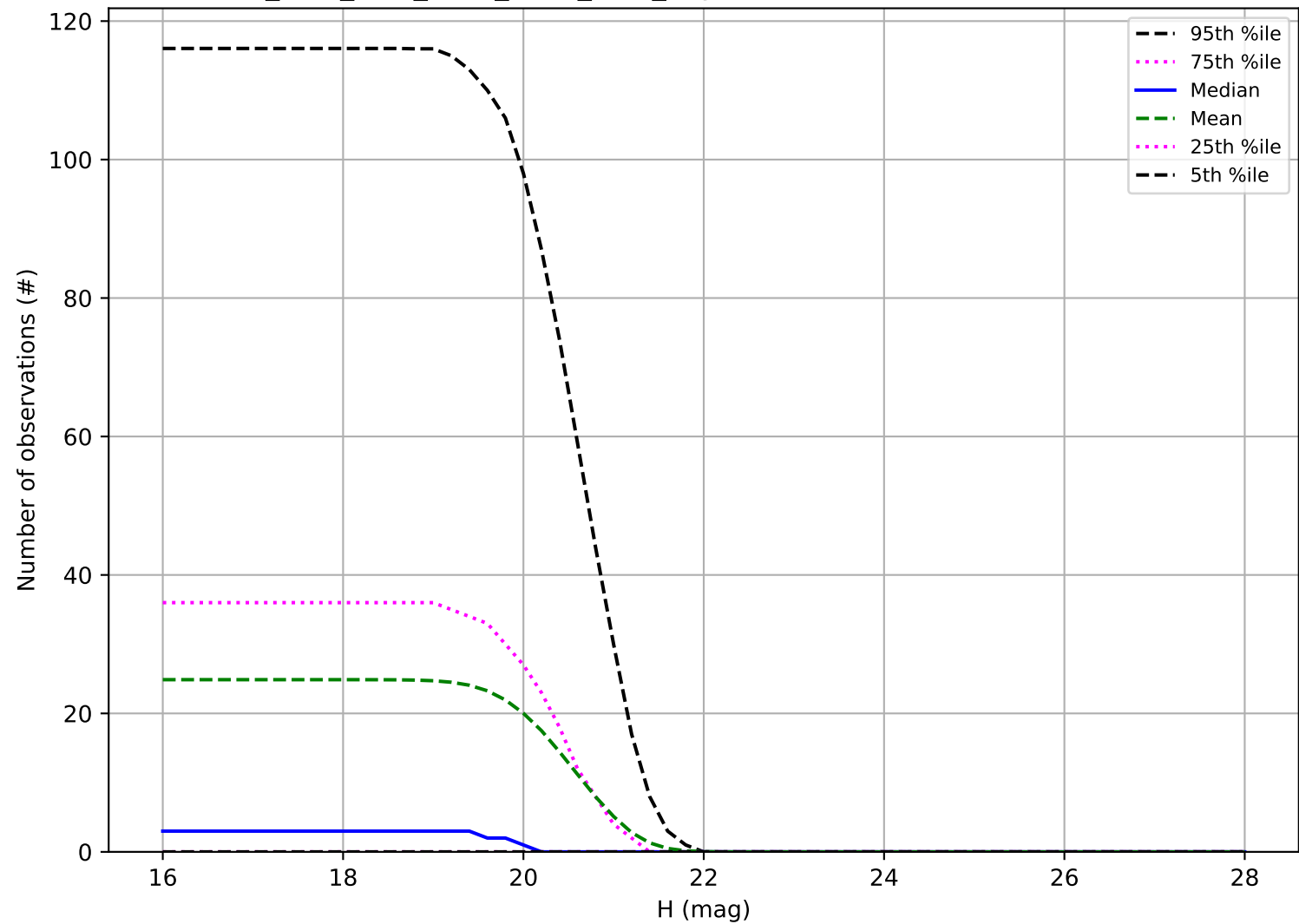
ddf_acor_sf15_lsf40_lsr20_v3.4_10yrs: Number of observations Vatira
