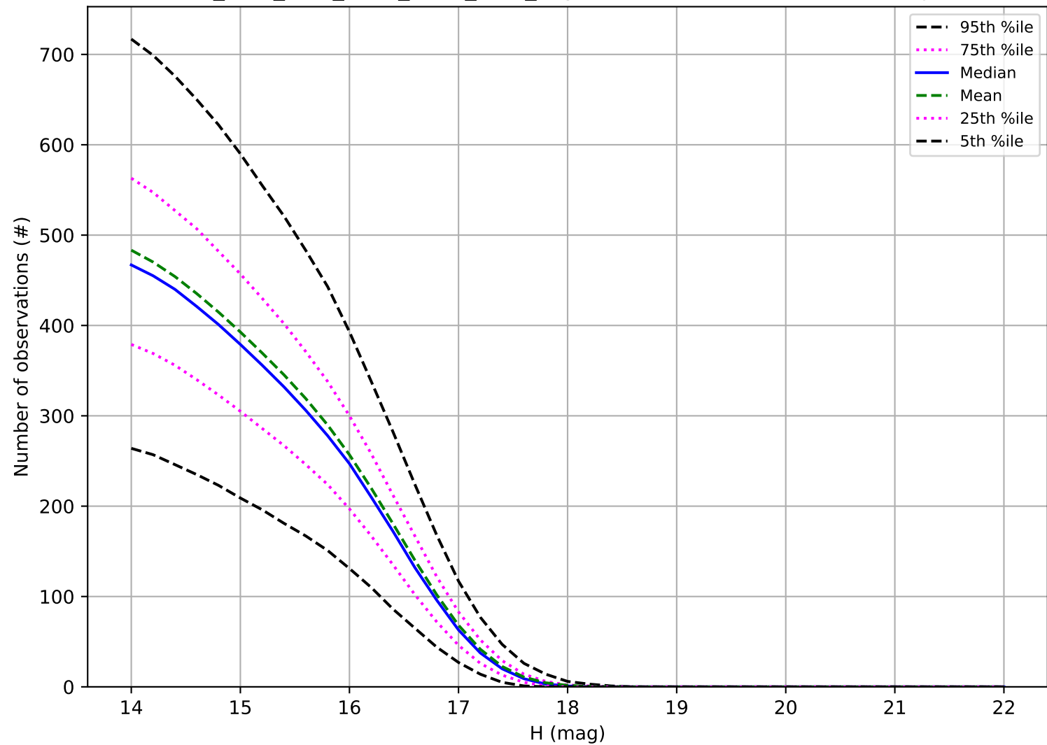
ddf_acor_sf15_lsf40_lsr20_v3.4_10yrs: Number of observations Trojan
