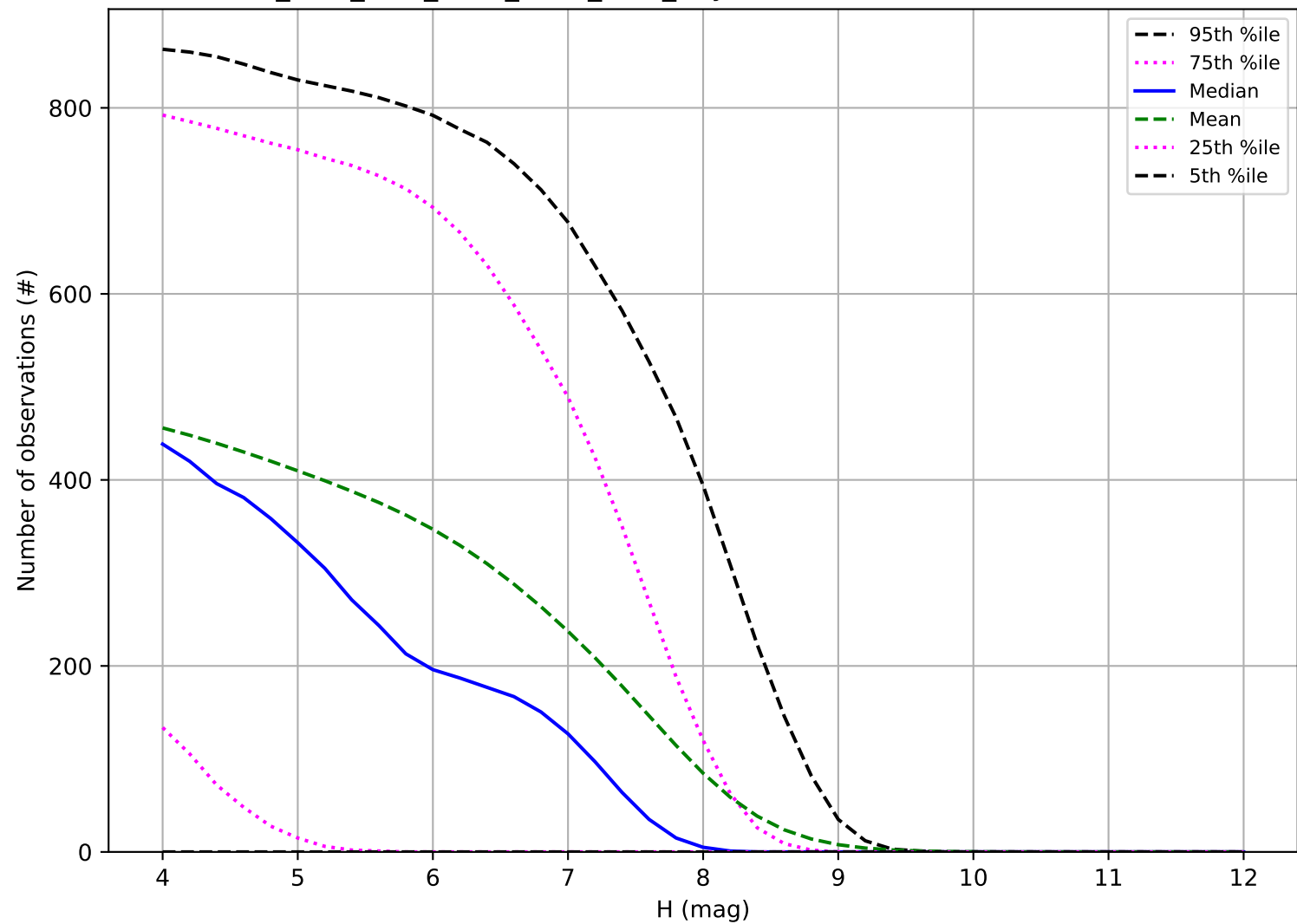
ddf_acor_sf15_lsf40_lsr20_v3.4_10yrs: Number of observations TNO
