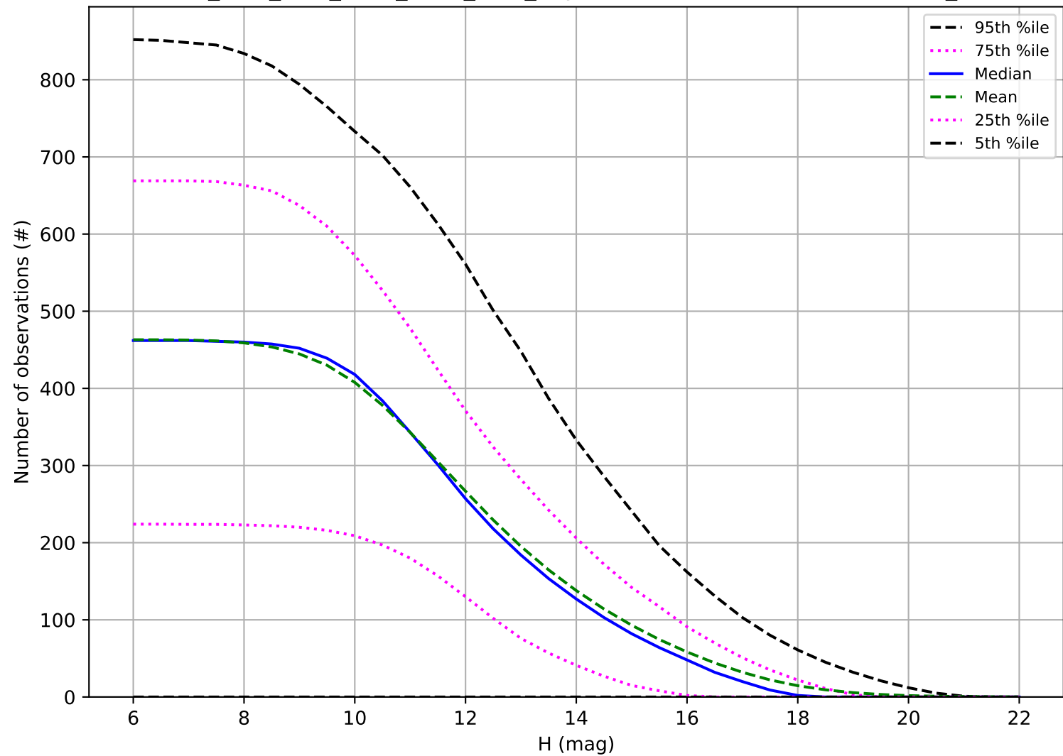
ddf_acor_sf15_lsf40_lsr20_v3.4_10yrs: Number of observations OCC_r5
