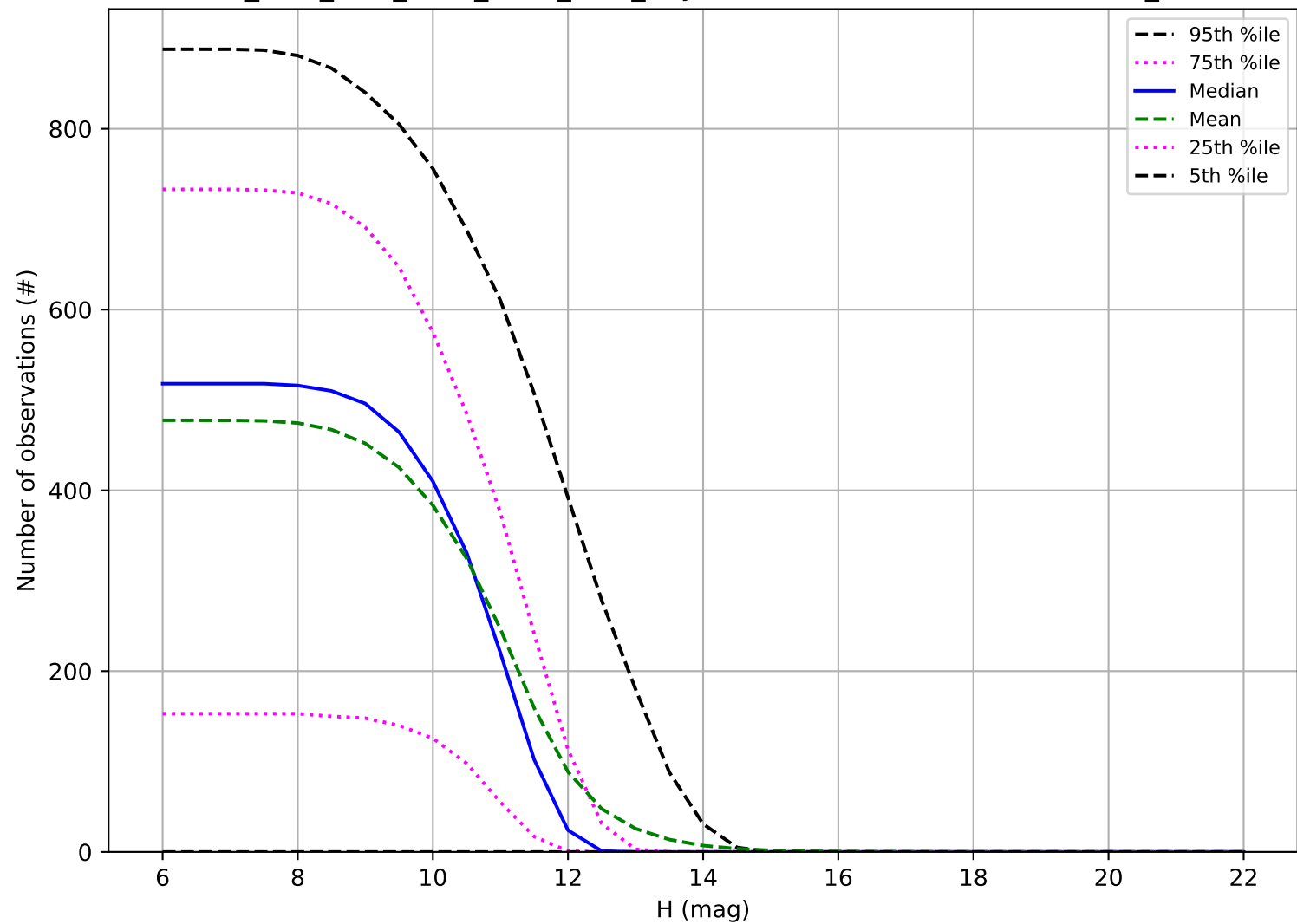
ddf_acor_sf15_lsf40_lsr20_v3.4_10yrs: Number of observations OCC_r20
