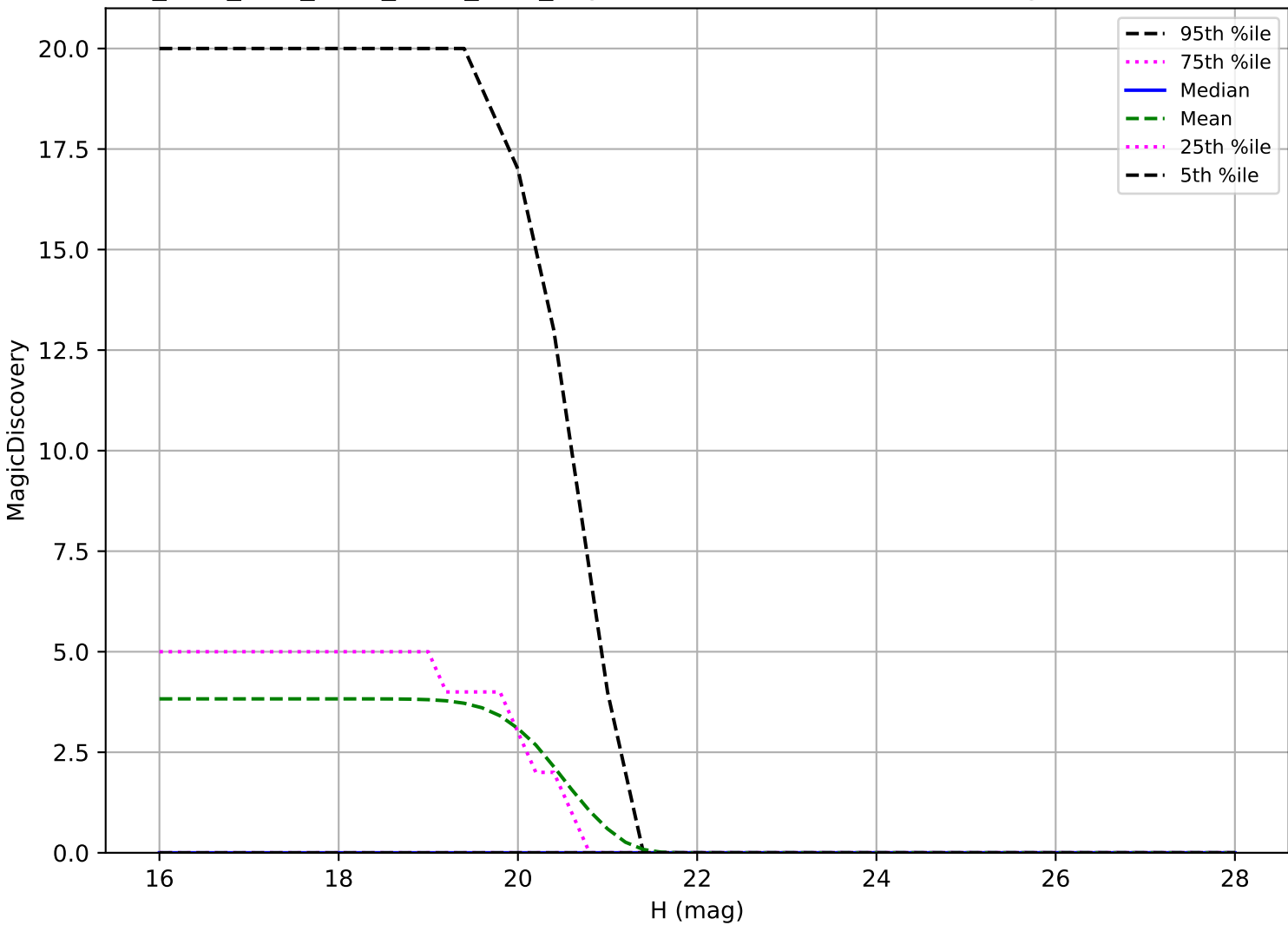
ddf_acor_sf15_lsf40_lsr20_v3.4_10yrs: Vatira 6 detections in 60 nights detection loss
