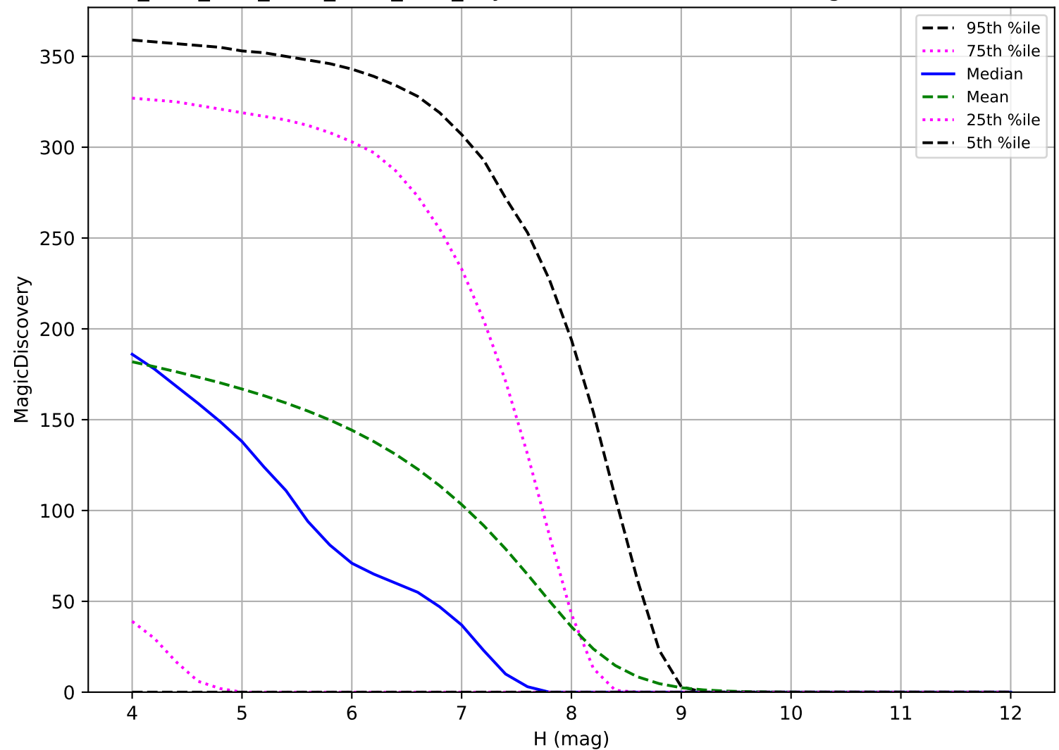
ddf_acor_sf15_lsf40_lsr20_v3.4_10yrs: TNO 6 detections in 60 nights detection loss
