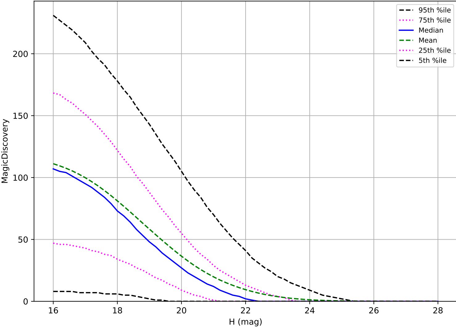
ddf_acor_sf15_lsf40_lsr20_v3.4_10yrs: PHA 6 detections in 60 nights detection loss
