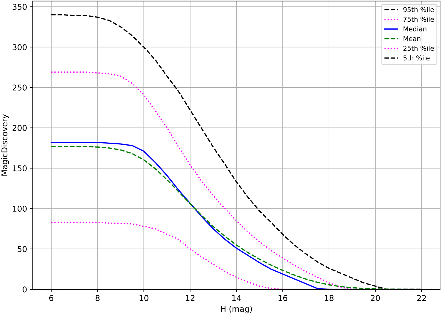
ddf_acor_sf15_lsf40_lsr20_v3.4_10yrs: OCC_r5 6 detections in 60 nights detection loss
