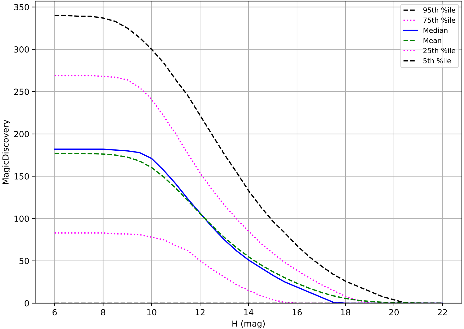
ddf_acor_sf15_lsf40_lsr20_v3.4_10yrs: OCC_r5 6 detections in 60 nights detection loss
