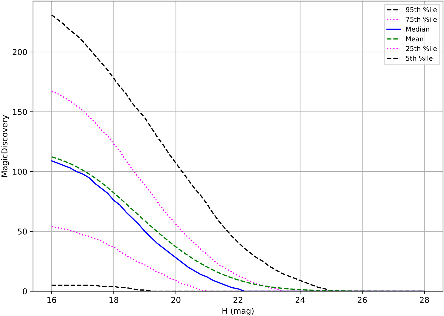
ddf_acor_sf15_lsf40_lsr20_v3.4_10yrs: NEO 6 detections in 60 nights detection loss
