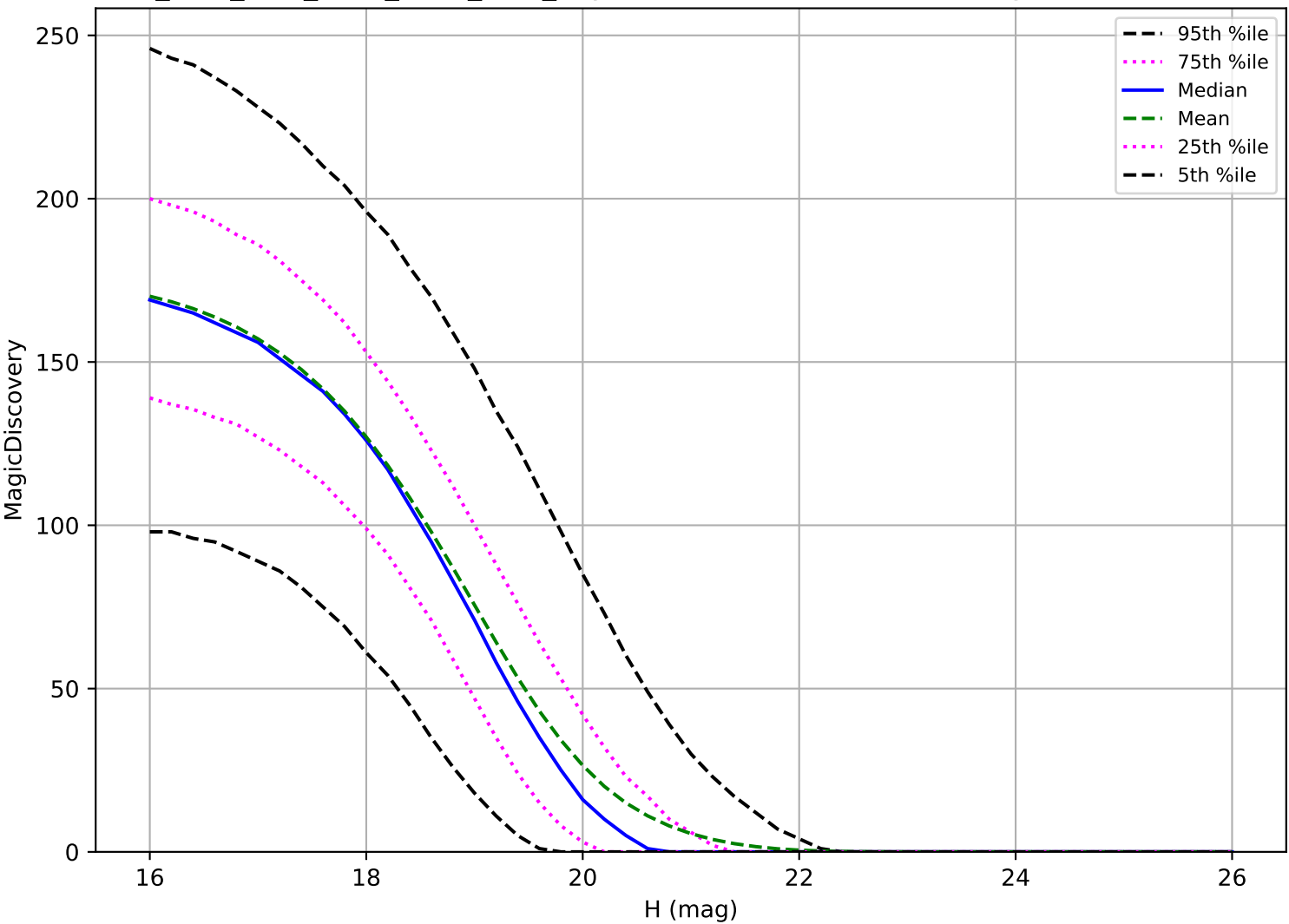
ddf_acor_sf15_lsf40_lsr20_v3.4_10yrs: MBA 6 detections in 60 nights detection loss
