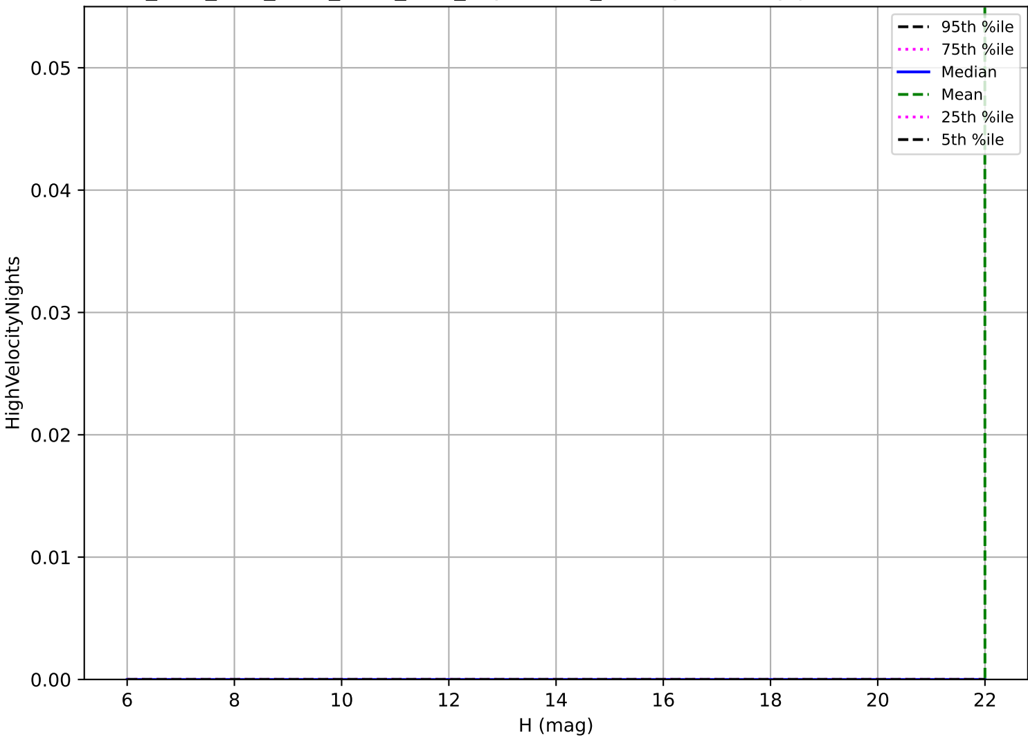
ddf_acor_sf15_lsf40_lsr20_v3.4_10yrs: OCC_r20 High velocity pair detection loss
