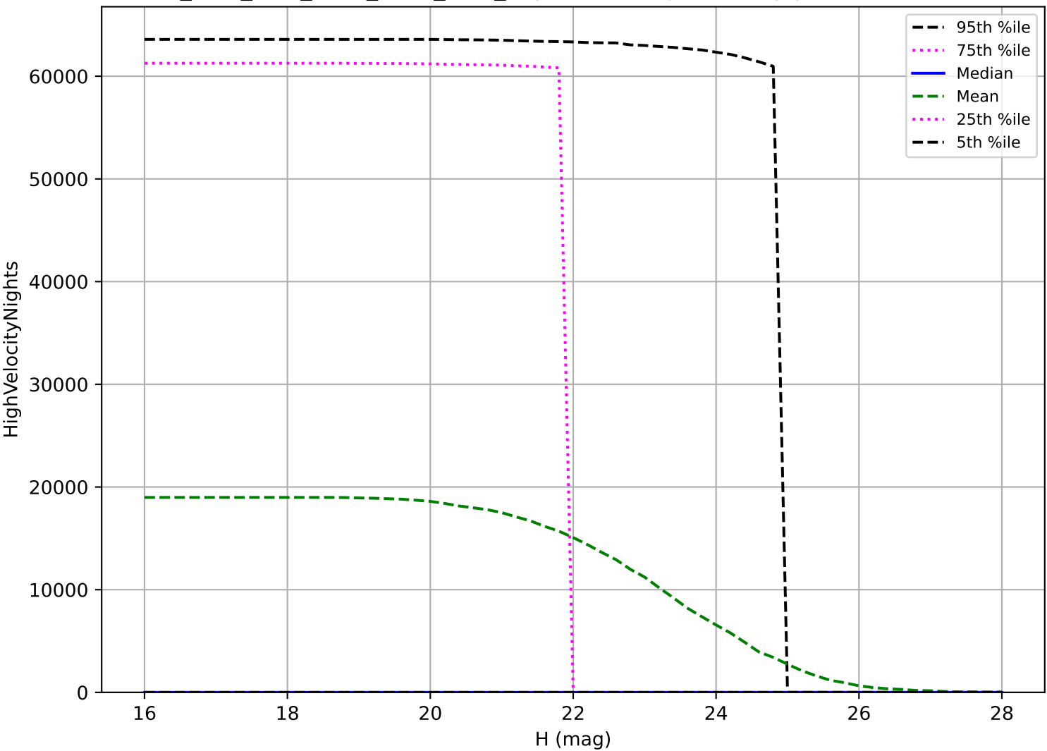
ddf_acor_sf15_lsf40_lsr20_v3.4_10yrs: NEO High velocity pair detection loss
