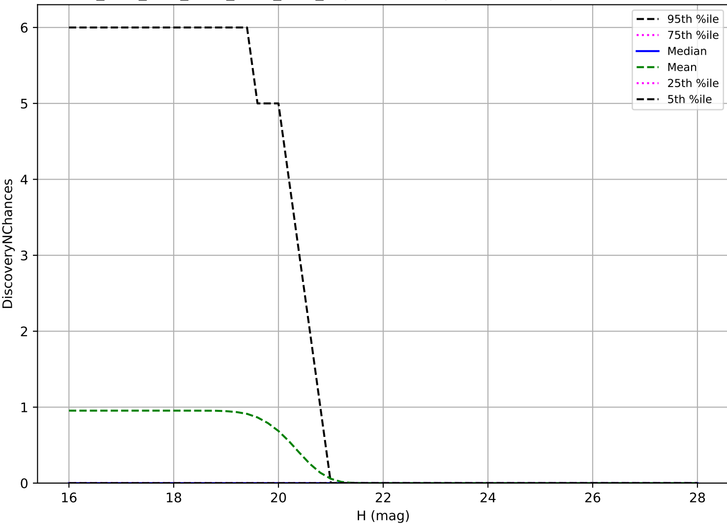
ddf_acor_sf15_lsf40_lsr20_v3.4_10yrs: Vatira 3 pairs in 15 nights detection loss
