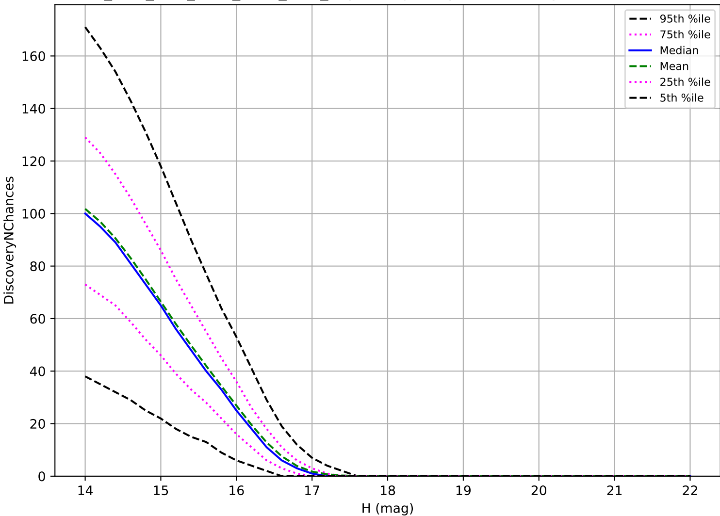
ddf_acor_sf15_lsf40_lsr20_v3.4_10yrs: Trojan 3 pairs in 15 nights detection loss
