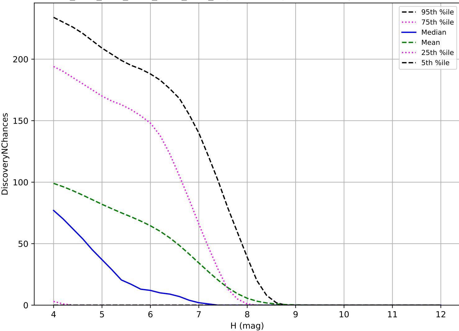
ddf_acor_sf15_lsf40_lsr20_v3.4_10yrs: TNO 3 pairs in 15 nights detection loss
