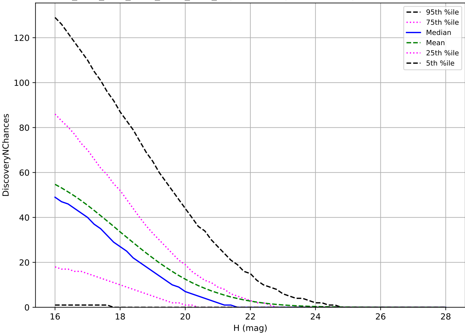
ddf_acor_sf15_lsf40_lsr20_v3.4_10yrs: PHA 3 pairs in 15 nights detection loss
