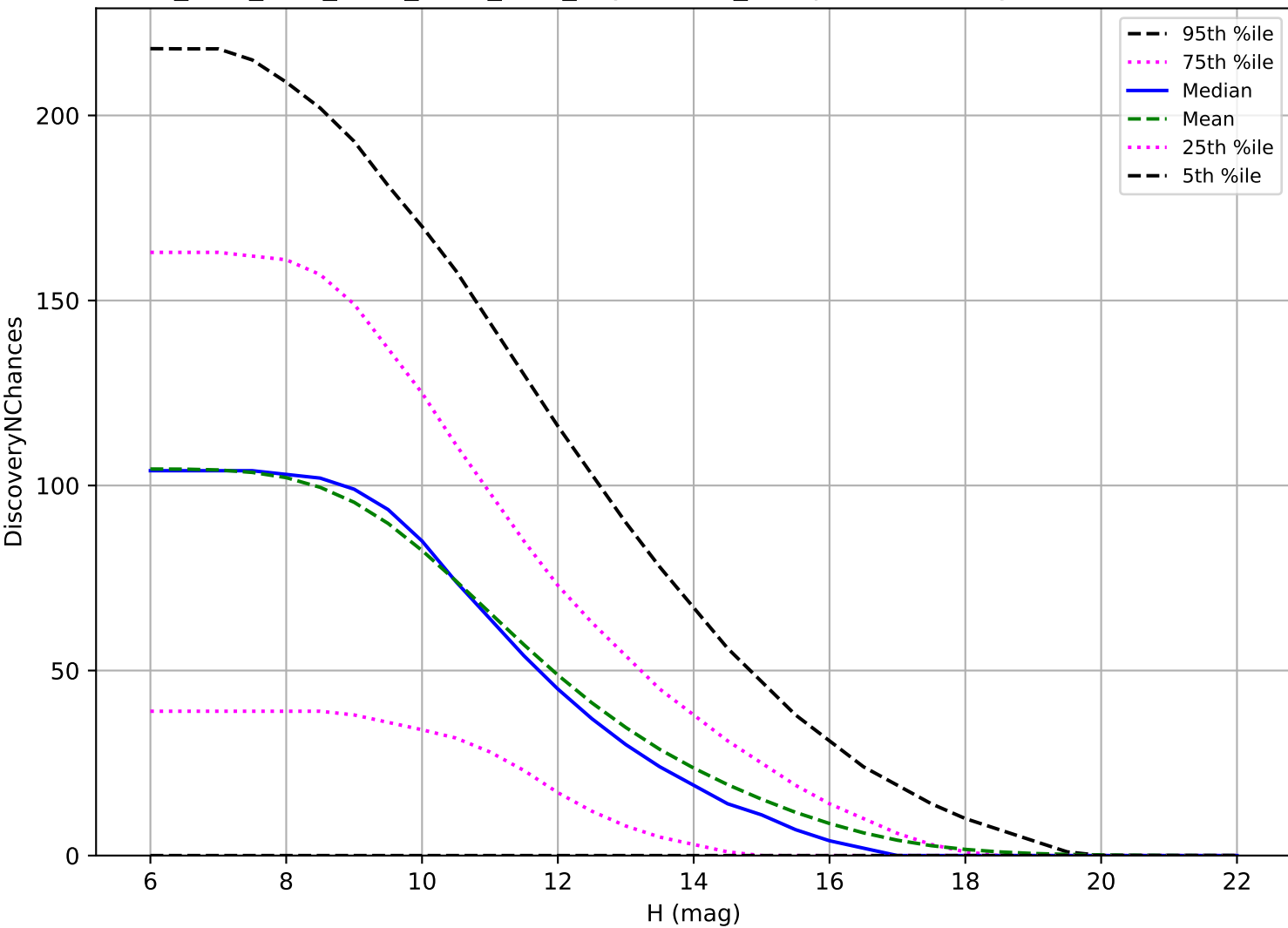
ddf_acor_sf15_lsf40_lsr20_v3.4_10yrs: OCC_r5 3 pairs in 15 nights detection loss
