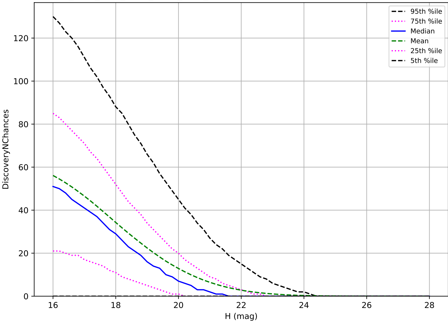
ddf_acor_sf15_lsf40_lsr20_v3.4_10yrs: NEO 3 pairs in 15 nights detection loss
