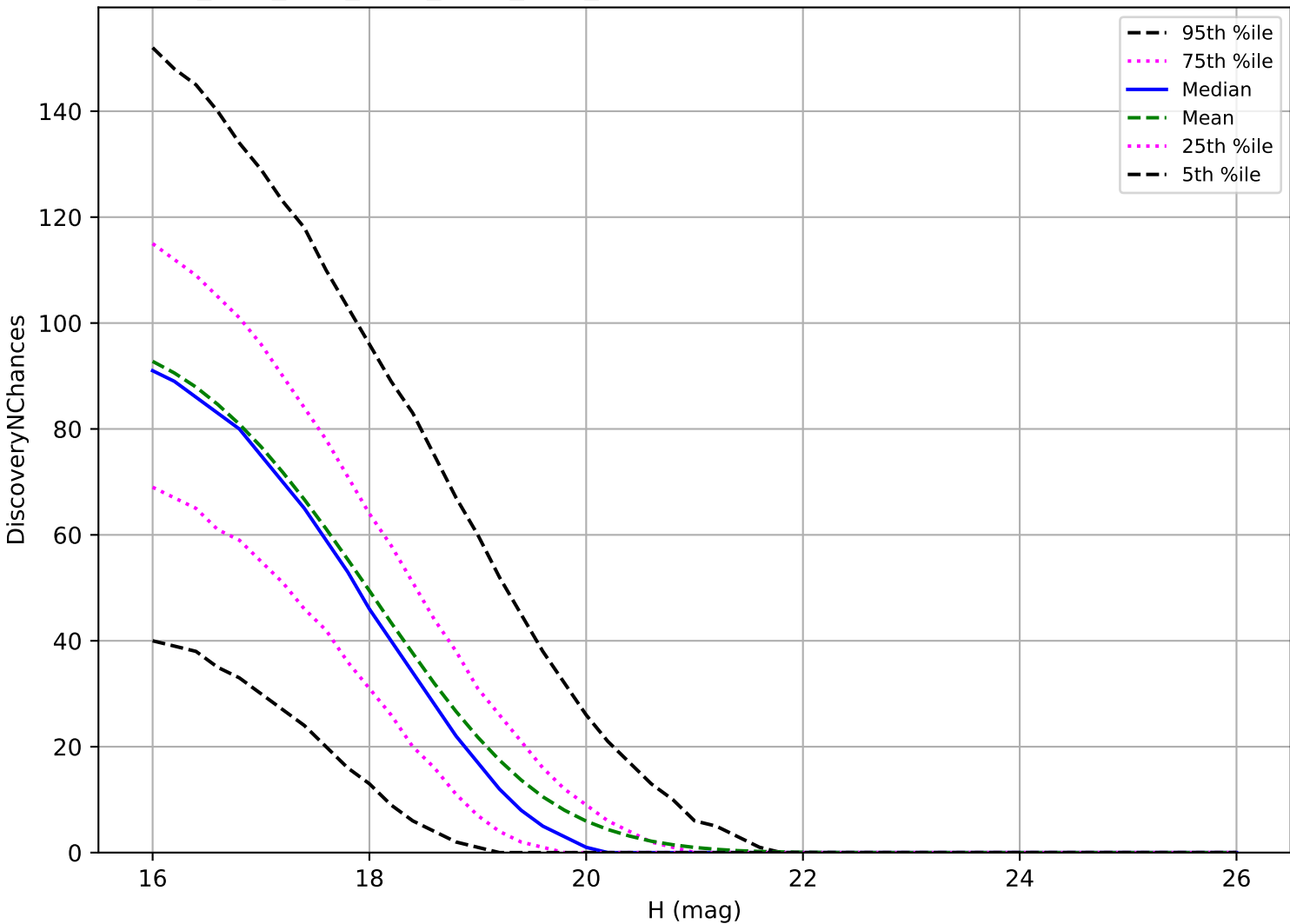
ddf_acor_sf15_lsf40_lsr20_v3.4_10yrs: MBA 3 pairs in 15 nights detection loss
