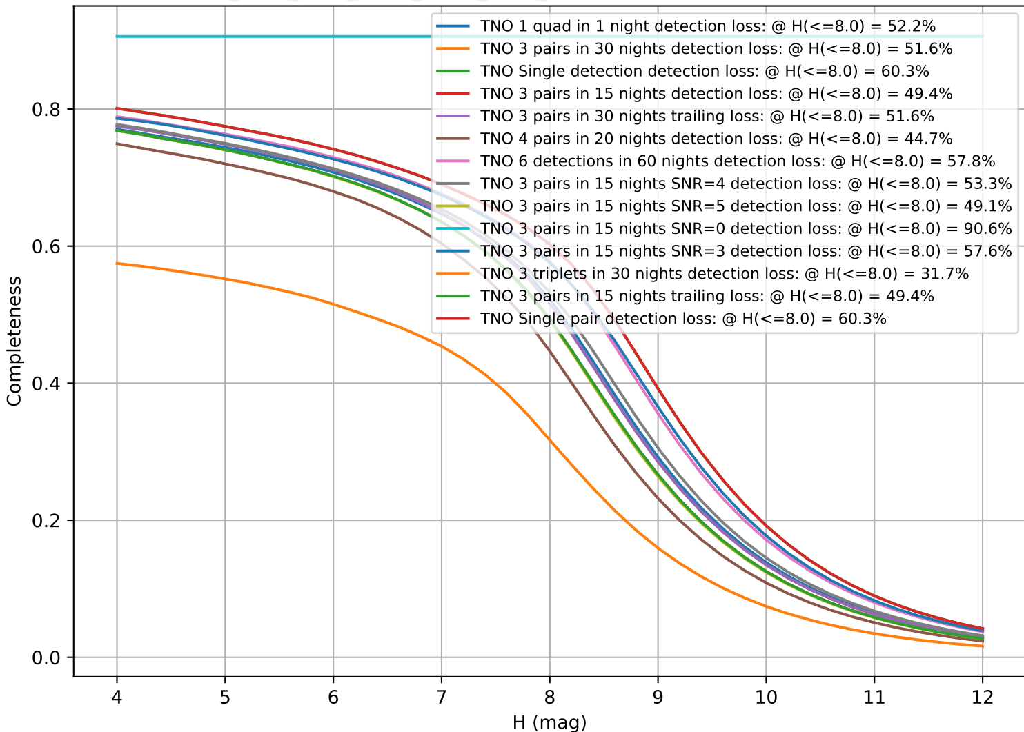
ddf_acor_sf15_lsf40_lsr20_v3.4_10yrs: CumulativeCompleteness
