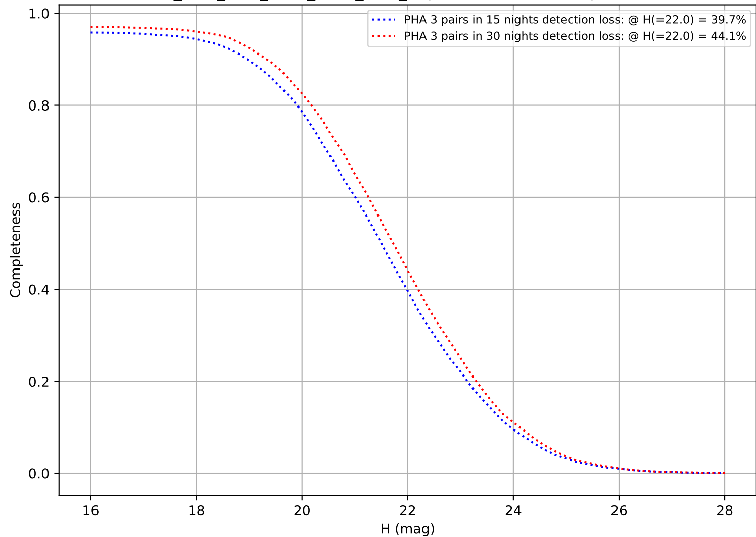
ddf_acor_sf15_lsf40_lsr20_v3.4_10yrs: DifferentialCompleteness
