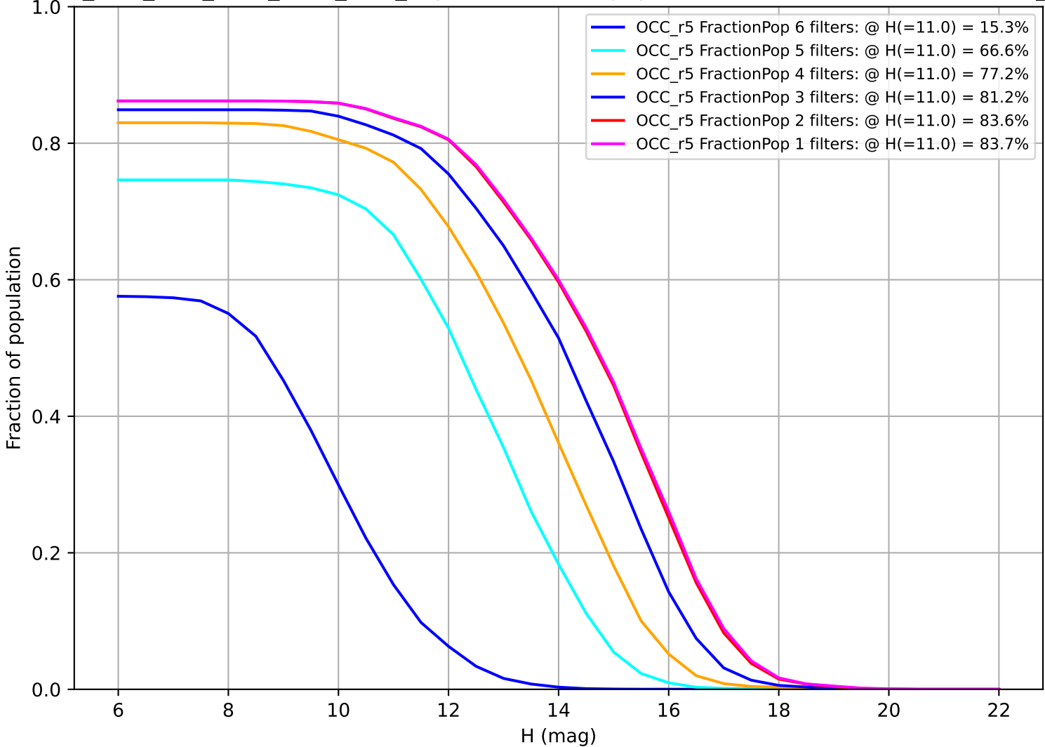
ddf_acor_sf15_lsf40_lsr20_v3.4_10yrs: Fraction of population with colors in X filters OCC_r5
