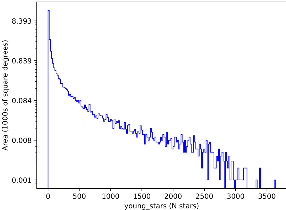
ddf_acor_sf15_lsf40_lsr20_v3.4_10yrs : young_stars
