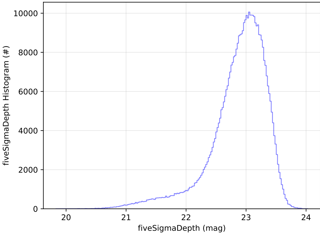
ddf_acor_sf15_lsf40_lsr20_v3.4_10yrs z: fiveSigmaDepth Histogram
