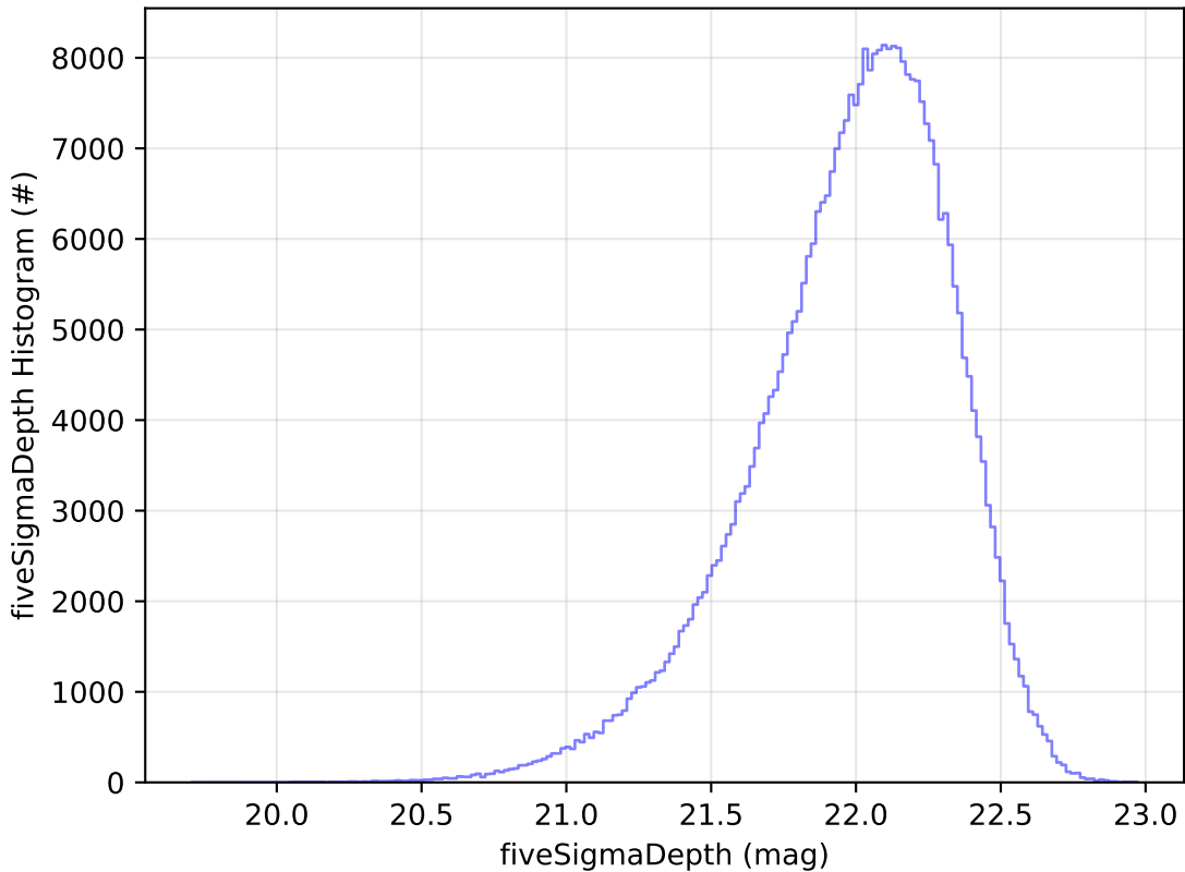
ddf_acor_sf15_lsf40_lsr20_v3.4_10yrs y: fiveSigmaDepth Histogram
