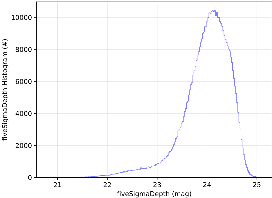
ddf_acor_sf15_lsf40_lsr20_v3.4_10yrs r: fiveSigmaDepth Histogram
