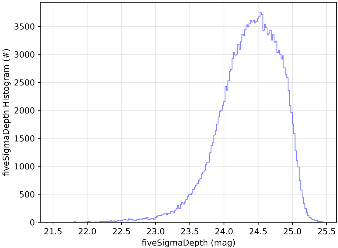
ddf_acor_sf15_lsf40_lsr20_v3.4_10yrs g: fiveSigmaDepth Histogram
