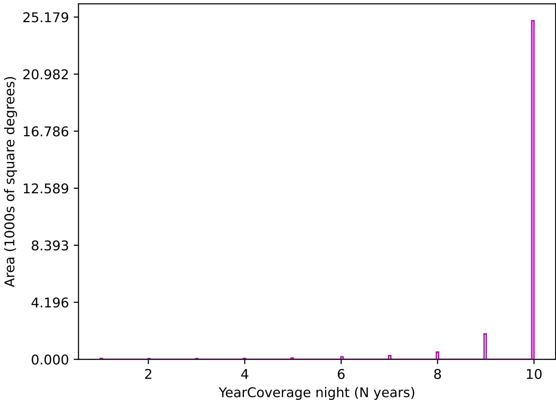
ddf_acor_sf15_lsf40_lsr20_v3.4_10yrs z band: YearCoverage night
