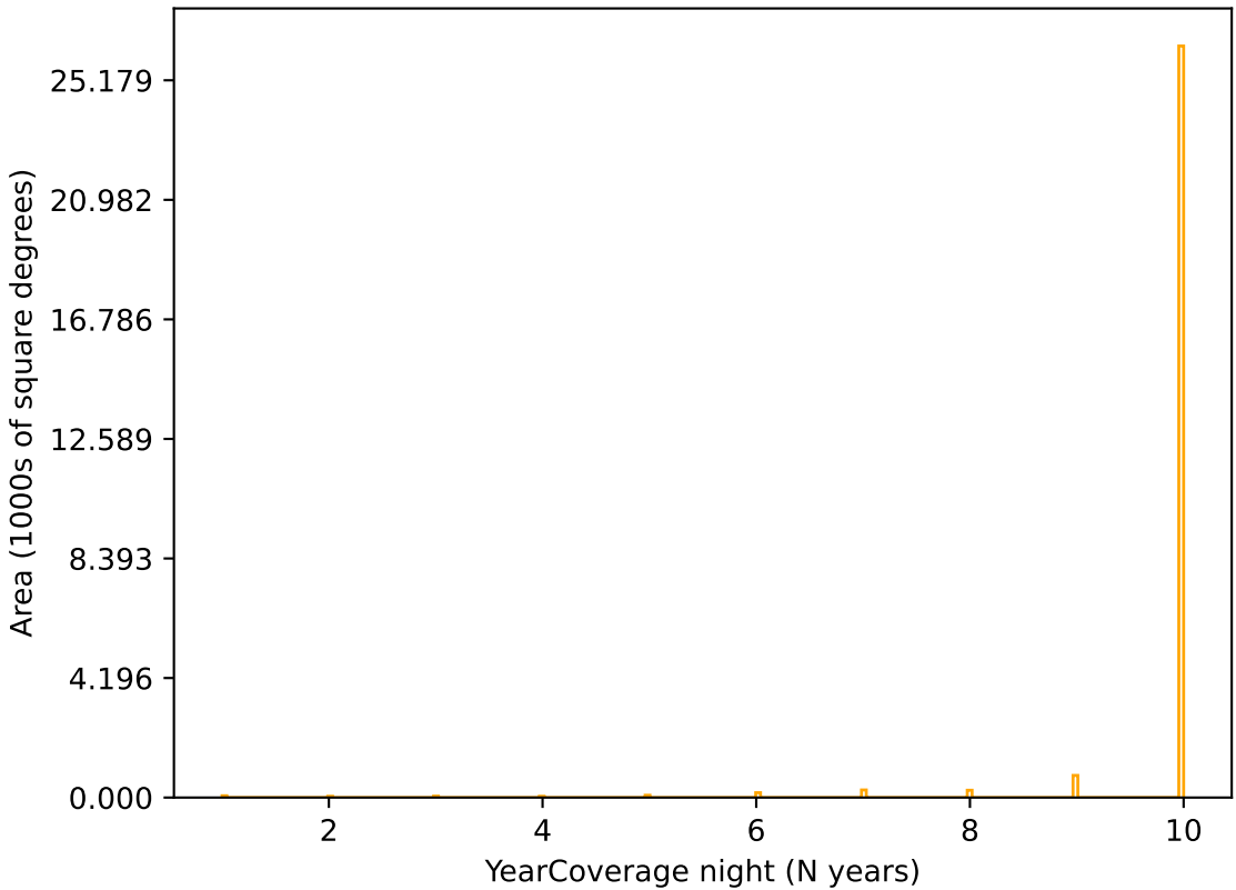
ddf_acor_sf15_lsf40_lsr20_v3.4_10yrs r band: YearCoverage night
