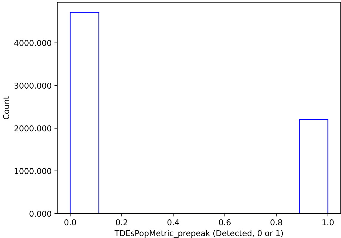
ddf_acor_sf15_lsf40_lsr20_v3.4_10yrs : TDEsPopMetric_prepeak
