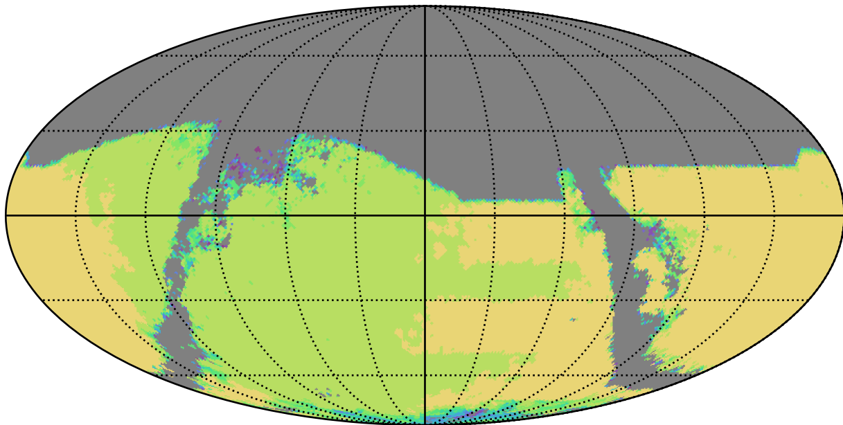
ddf_acor_sf15_lsf40_lsr20_v3.4_10yrs : TDC_campaign
