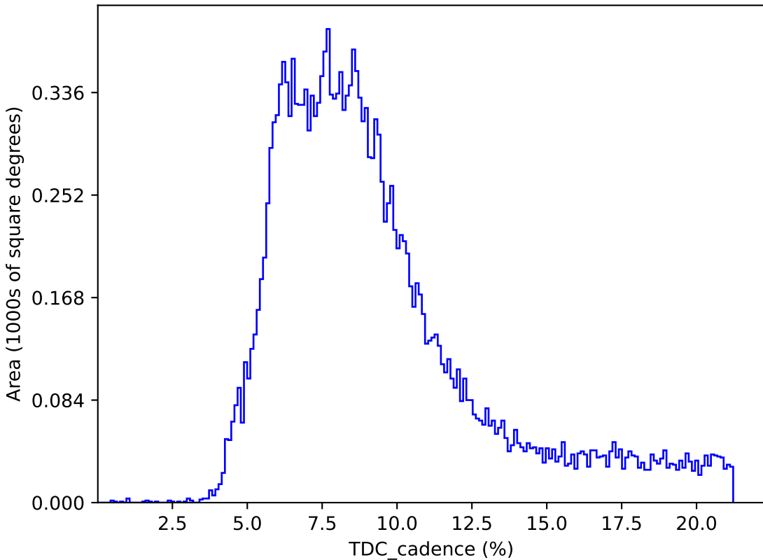
ddf_acor_sf15_ls40_lsr20_v3.4_10yrs : TDC_cadence
