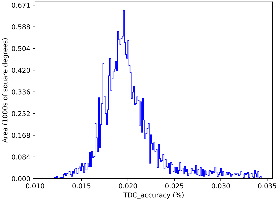
ddf_acor_sf15_ls40_lsr20_v3.4_10yrs : TDC_accuracy
