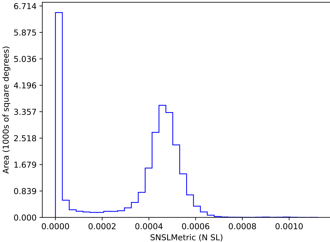
ddf_acor_sf15_lsf40_lsr20_v3.4_10yrs : SNSLMetric
