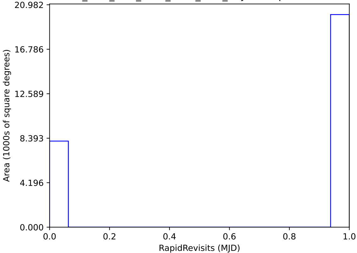
ddf_acor_sf15_lsf40_lsr20_v3.4_10yrs : RapidRevisits
