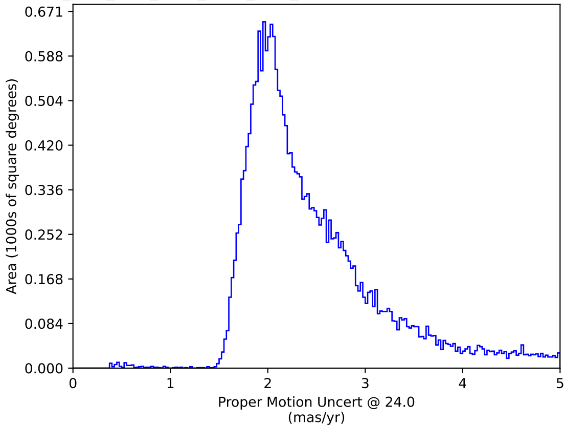
ddf_acor_sf15_lsf40_lsr20_v3.4_10yrs : Proper Motion Uncert @ 24.0
