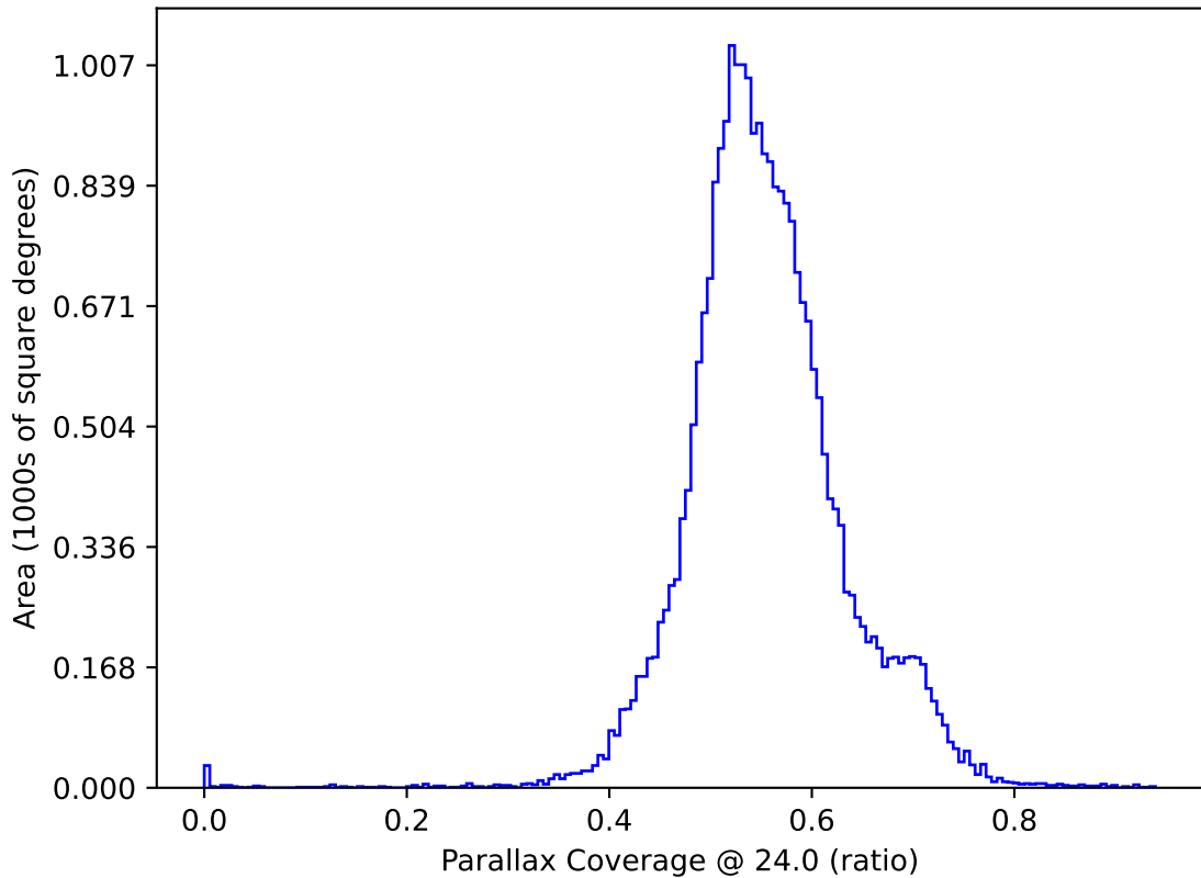
ddf_acor_sf15_lsf40_lsr20_v3.4_10yrs : Parallax Coverage @ 24.0
