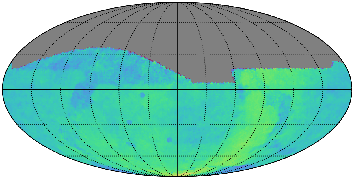
ddf_acor_sf15_lsf40_lsr20_v3.4_10yrs : Parallax Coverage @ 22.4
