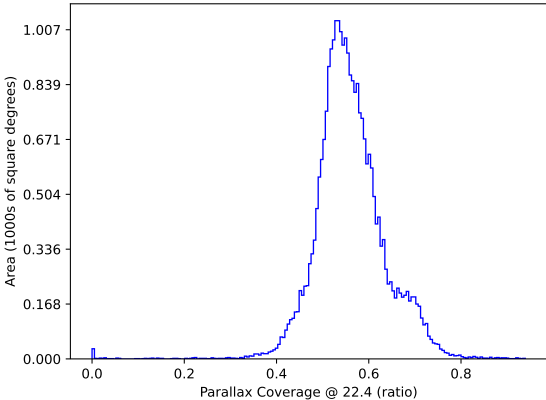
ddf_acor_sf15_lsf40_lsr20_v3.4_10yrs : Parallax Coverage @ 22.4
