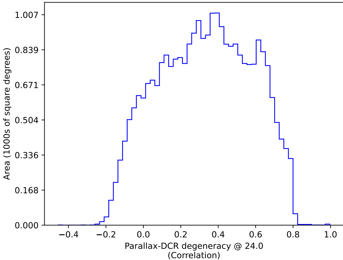
ddf_acor_sf15_lsf40_lsr20_v3.4_10yrs : Parallax-DCR degeneracy @ 24.0
