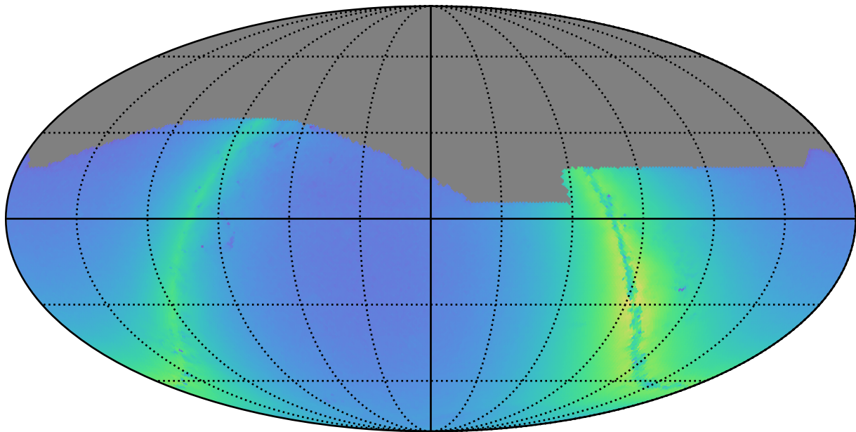
ddf_acor_sf15_lsf40_lsr20_v3.4_10yrs r: Nstars_no_crowding
