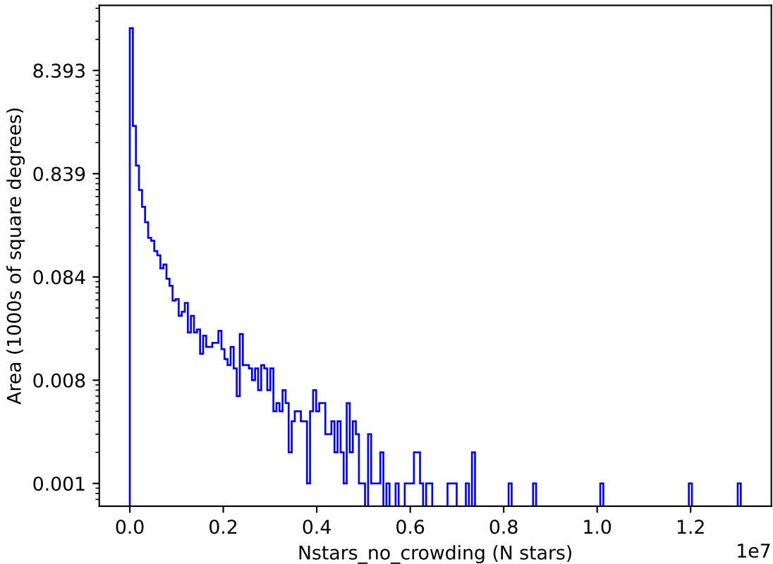
ddf_acor_sf15_lsf40_lsr20_v3.4_10yrs g: Nstars_no_crowding
