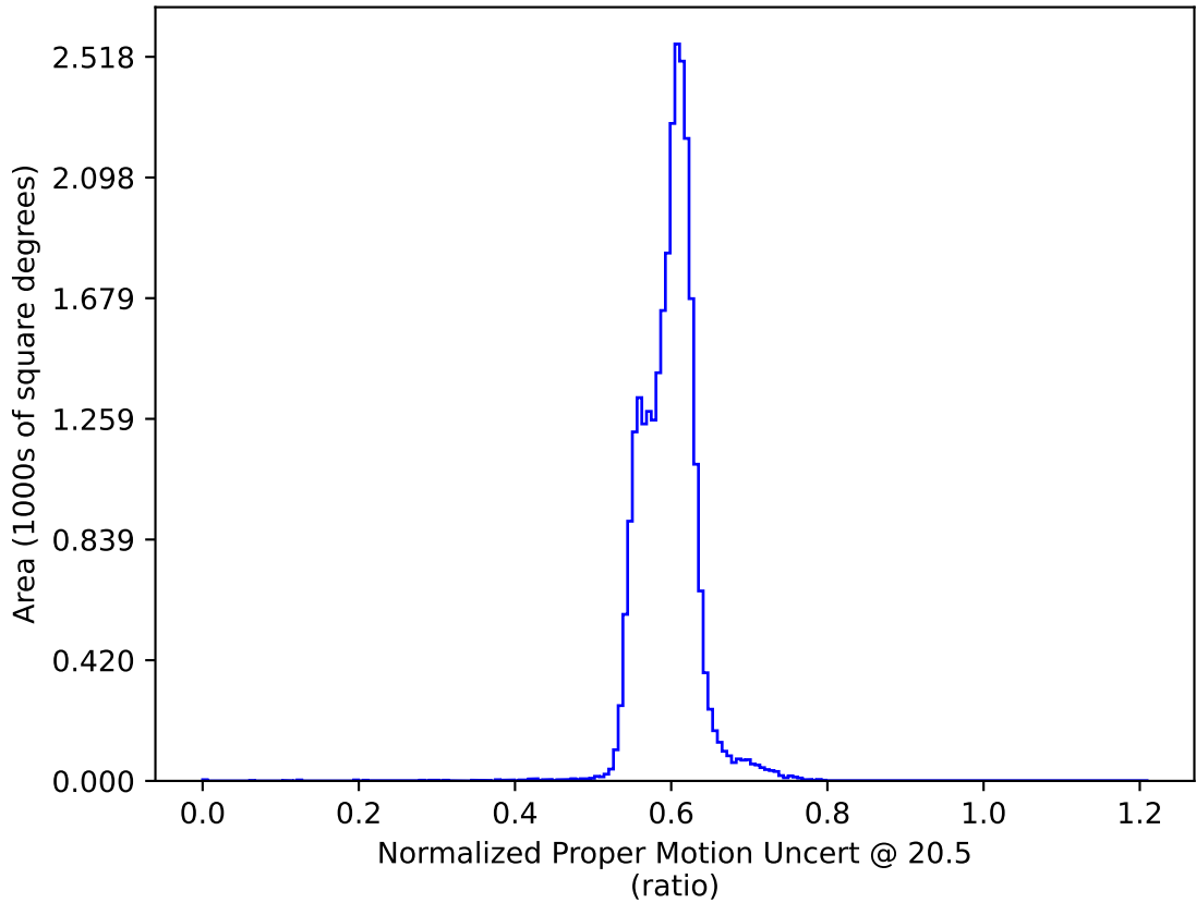
ddf_acor_sf15_lsf40_lsr20_v3.4_10yrs : Normalized Proper Motion Uncert @ 20.5
