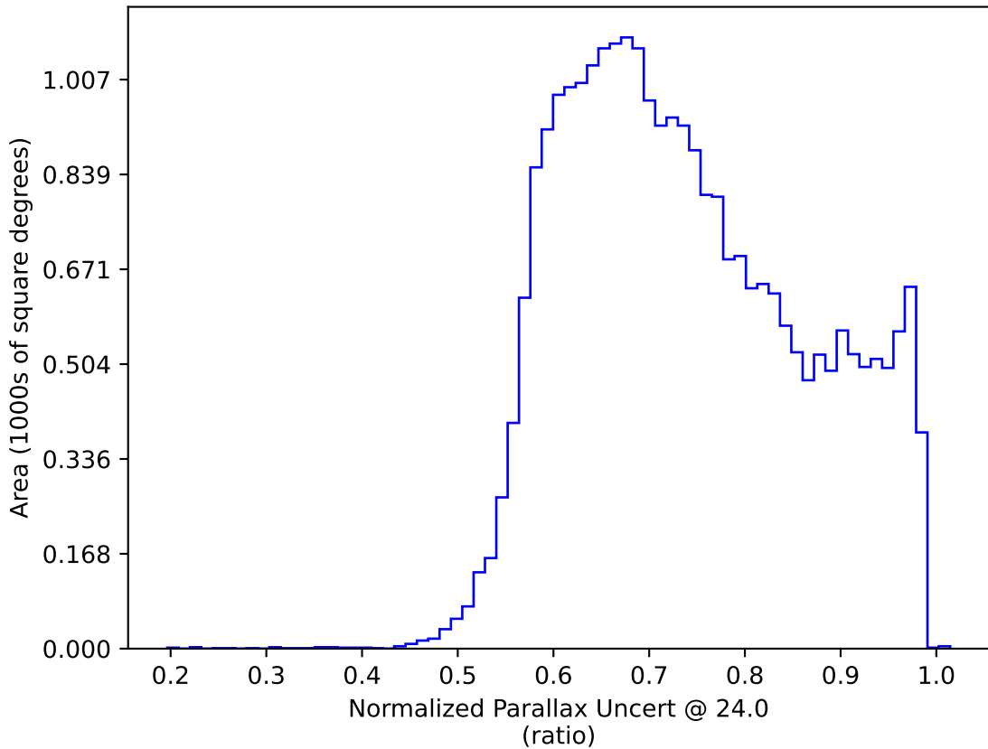
ddf_acor_sf15_lsf40_lsr20_v3.4_10yrs : Normalized Parallax Uncert @ 24.0
